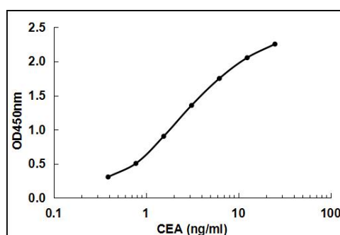
Figure 1. Sandwich ELISA using KT159 as capture antibody and HRP conjugated KT160 as detection antibody
